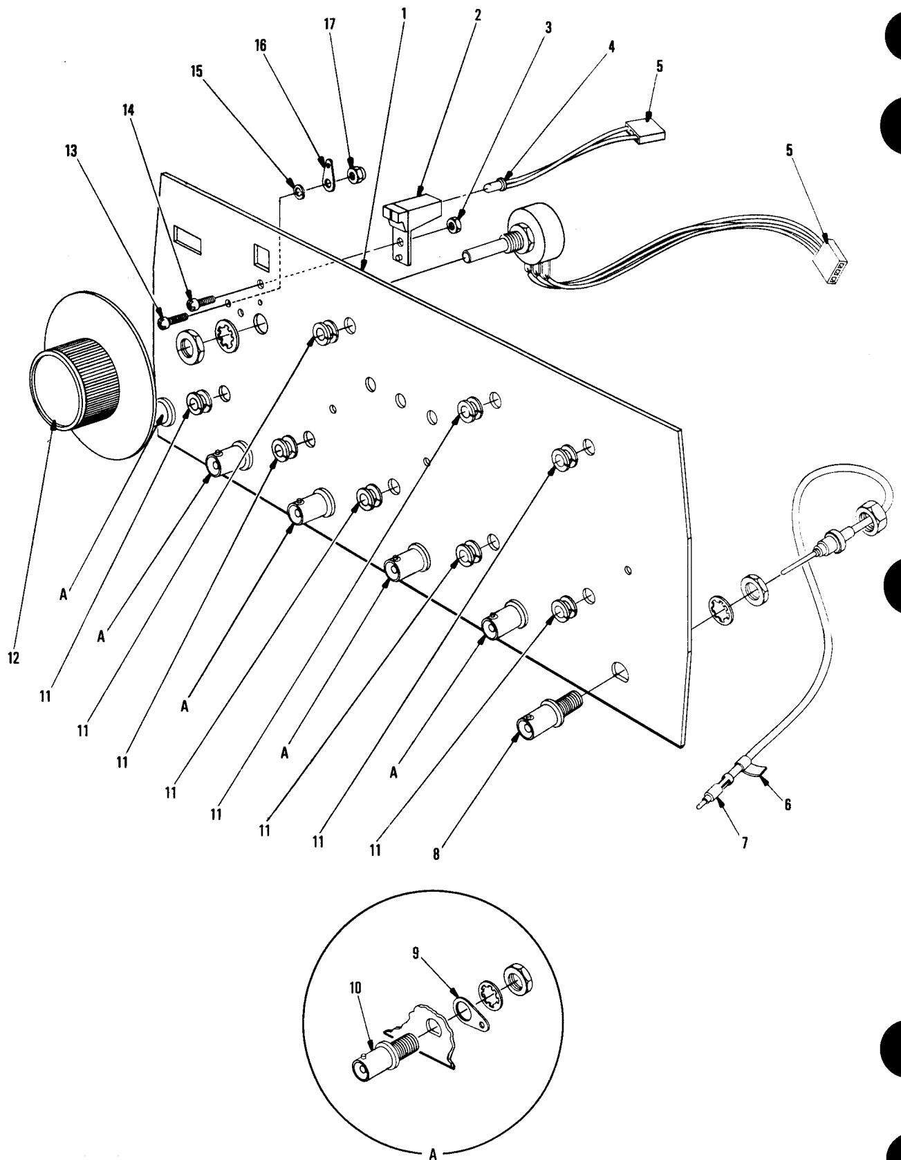
Figure 4. Front Panel Assembly.
