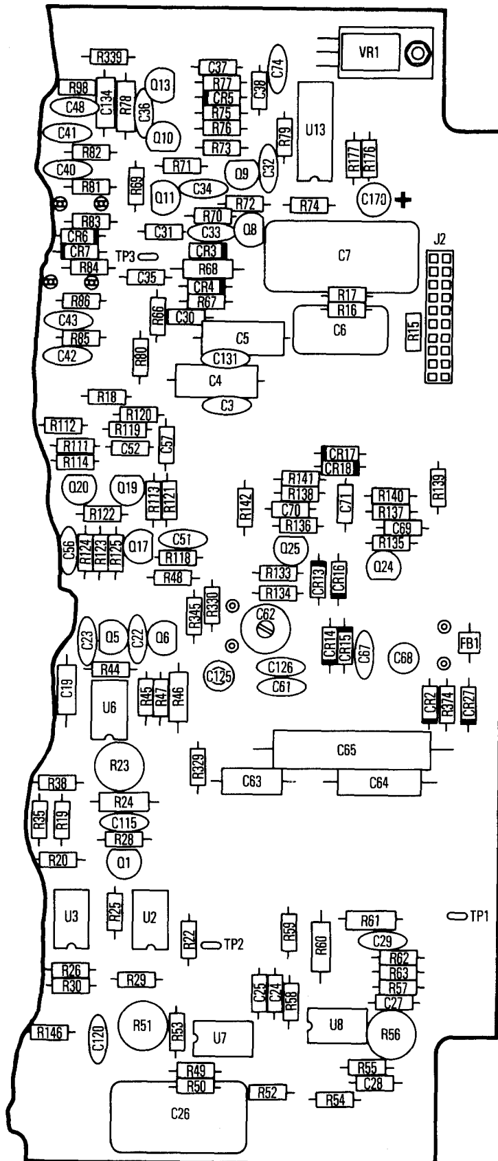
Figure 2. Main Board Assembly (Sheet 4 of 4).
