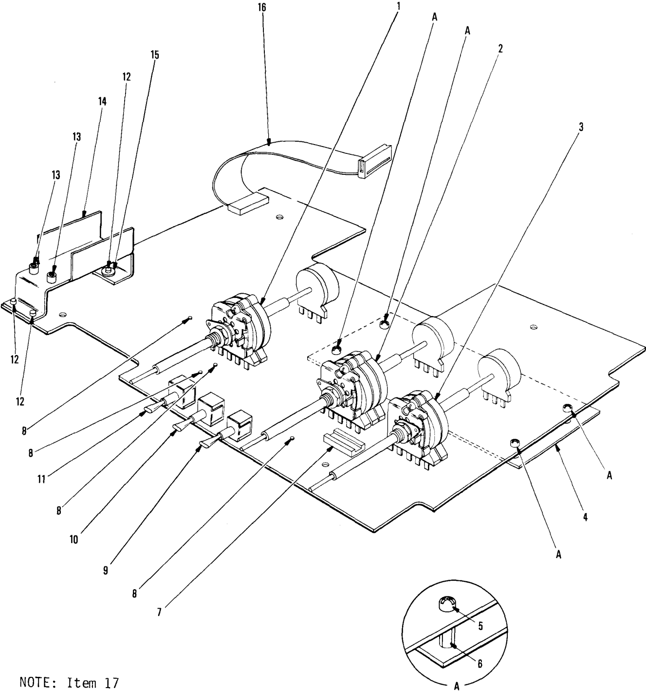
Figure 3. Auxiliary Board Assembly (Sheet 1 of 3).
