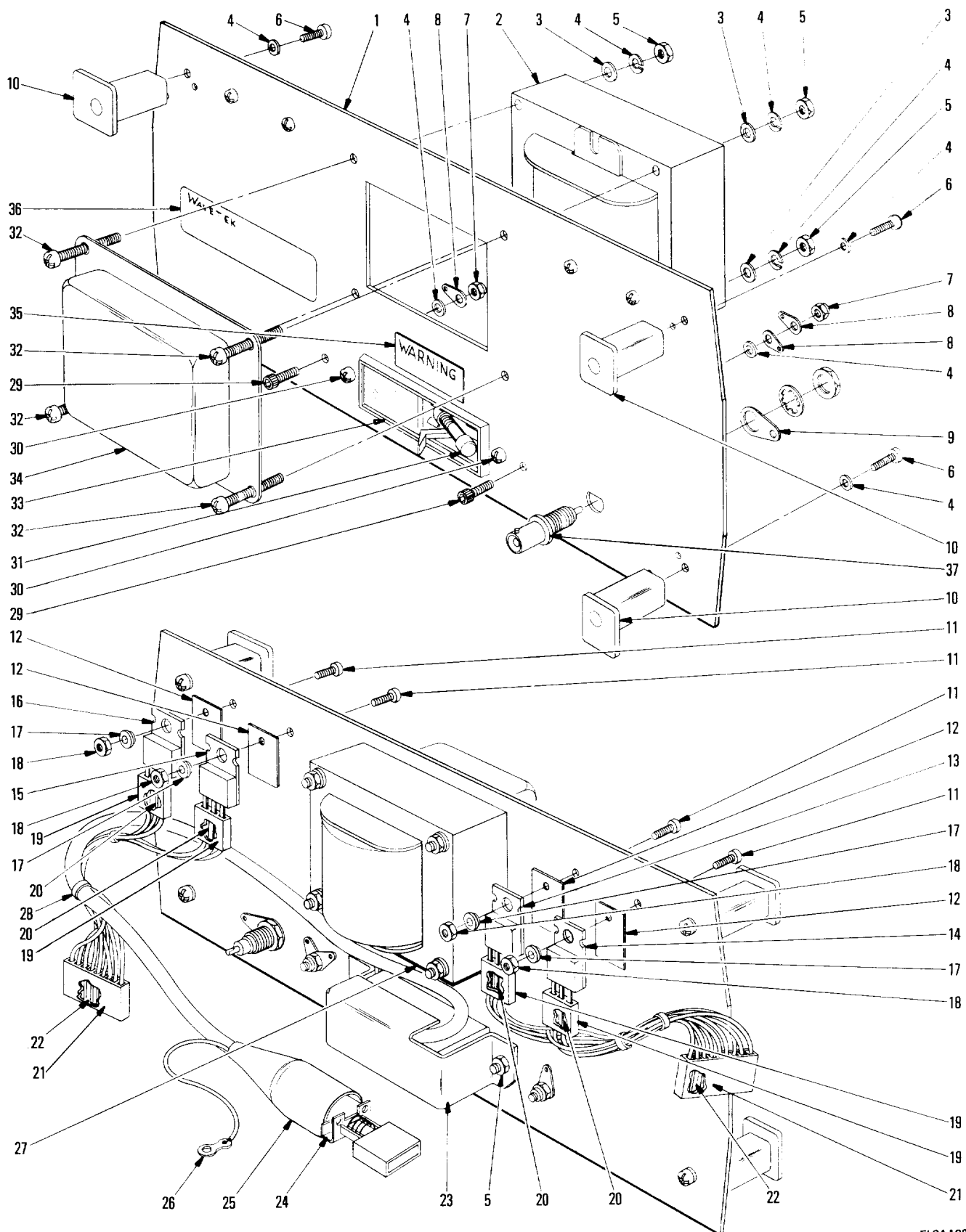
Figure 5. Rear Panel Assembly.
