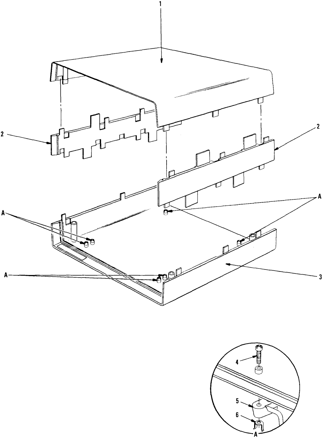
Figure 6. Cover Assembly.
